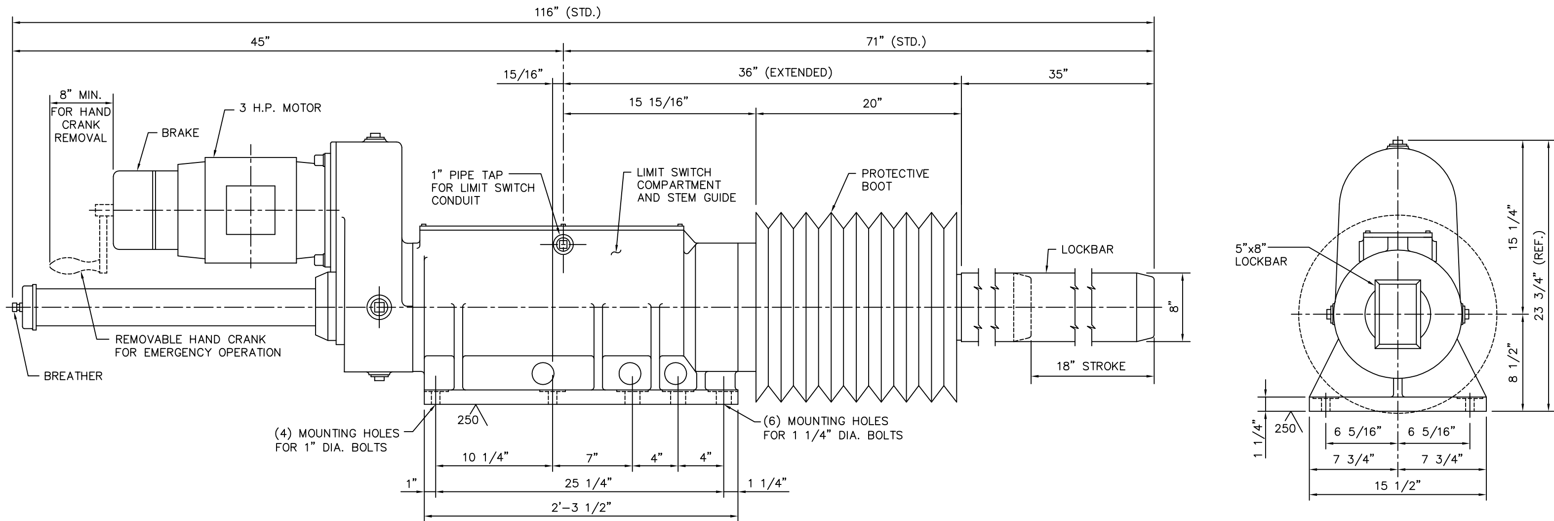
EARLE ® EG-3 LOCKBAR OPERATOR
